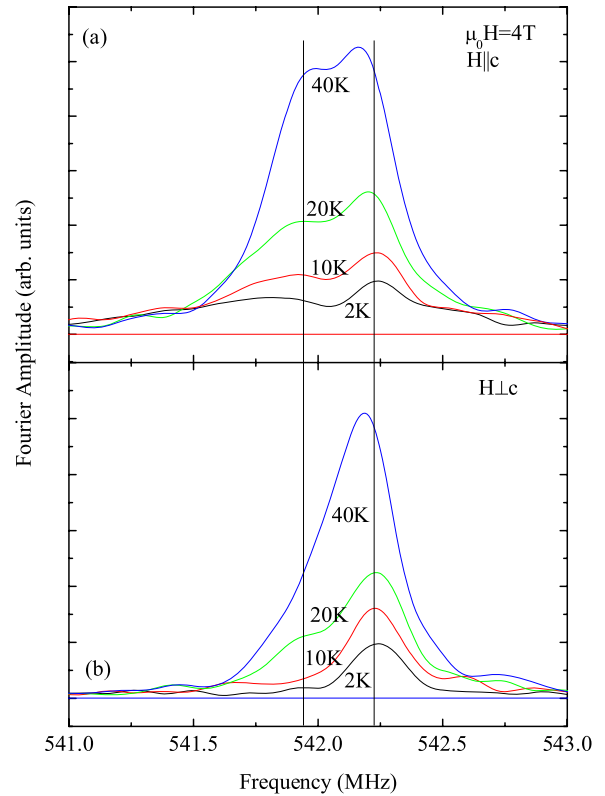
Figure 2. The temperature dependence of the Fourier transform of the \mu SR asymmetry data in a field of 4 T. (a) The spectra obtained when the field \vec{H} is parallel to the \hat{c} axis, which is normal to the mosaic (and thus to the kagome plane). (b) The spectra obtained when the field \vec{H} is perpendicular to the \hat{c} axis.
