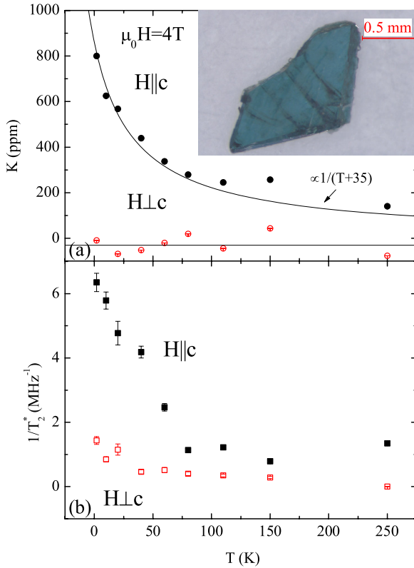
Figure 1. The temperature dependence of (a) the muon frequency shift K (errors are smaller than the symbol) and (b) relaxation rate 1/T_2^* for two orientations of the crystals (filled symbols for \vec{H} \parallel \hat{c} and hollow for \vec{H} \perp \hat{c} ). The solid line represent a Curie-Weiss-type law. The inset shows a typical crystal.
