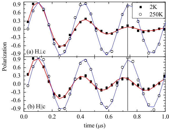
Figure 3. \mu SR data in the time domain using a rotating reference frame of 539 MHz, for the two different field directions and two different temperatures: 250 and 2 K. (a) \vec{H} \perp \hat{c} ; no shift is detected between the two temperatures, but an increase in relaxation is observed. (b) \vec{H} \parallel \hat{c} ; a shift in the frequency and increase in relaxation are observed. The solid lines are fits of equation (1) to the data. The solid vertical line shows when a shift is present and when it is not.
