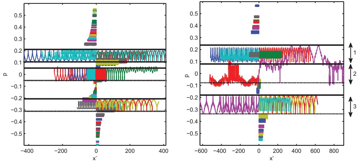
Figure 1. A phase-space portrait for three resonances. Different colors (shades) describe different trajectories. The horizontal black solid and dashed lines designate the edges of the resonance chains. The initial conditions were uniformly distributed on the p -axis ( x(t=0) = 0 ). The system was integrated up to t = 10^4 (dimensionless variables). At the left figure three non-overlapping resonances are presented, while in the right figure resonances (1) and (2) overlap.
