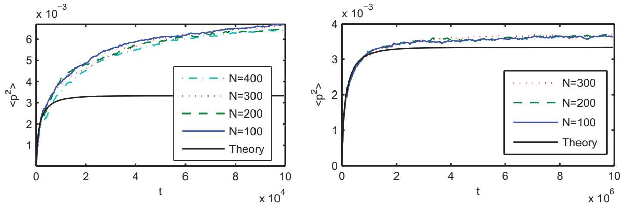
Figure 2. \langle p^2 \rangle as a function of t . Dashed gray lines are the numerical solution of (44) for 1000 initial conditions taken from a Gaussian distribution. Different shades and styles of lines designate different N (see legend). The solid thick black lines are the numerical solutions of (53) with a diffusion constant given by (52). The parameters are k_R = 0.1 and \sigma = 10^{-3} for the left figure and \sigma = 10^{-4} for the right figure.
