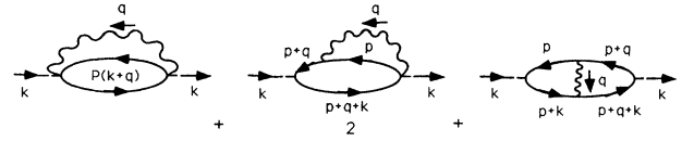
FIG. 8. Diagrams contributing to the correlations of the GPFPG (Appendix C).
