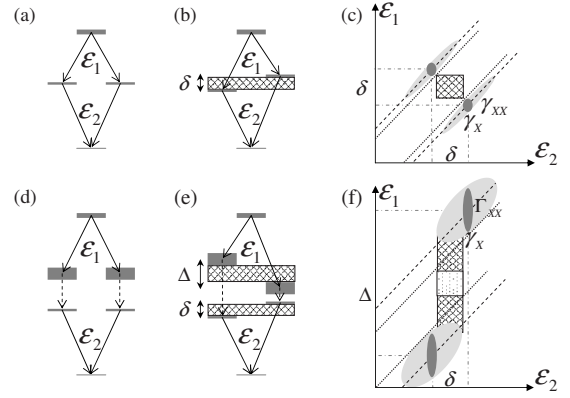
FIG. 4. (a) Ideal direct cascade. The widths of the levels represent their decay rate. (b) Ground-state biexciton cascade in an anisotropic QD. (c) Schematic two-photon probability distribution. Dark gray—high probability areas. Cross hatched—spectral filter. Light gray—inhomogeneous broadening due to spectral diffusion. [(d)–(f)] Same as (a)–(c) (respectively), for an indirect cascade. In (e) and (f) only the case of splittings in opposite directions is shown. The dotted rectangle in (f) is an example for a filter not penetrated by the high-probability areas for any amount of spectral diffusion.
