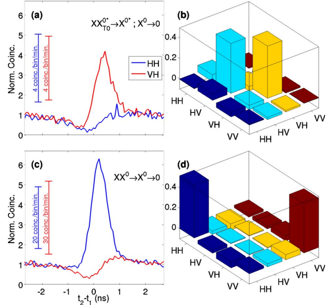
FIG. 2. (Color online) [(a) and (c)] Measured intensity correlation functions for the spin-blockaded and ground-state biexciton cascades, respectively. Blue (dark-gray) [red (light-gray)] line represents the correlation in co-[cross-]linear polarizations. The coincidence rates are indicated by the scale bars in units of coincidences per time bin (80 ps) per minute. [(b) and (d)] Real parts of the two-photon polarization density matrices measured for the spin-blockaded and ground-state biexciton cascades, respectively.
