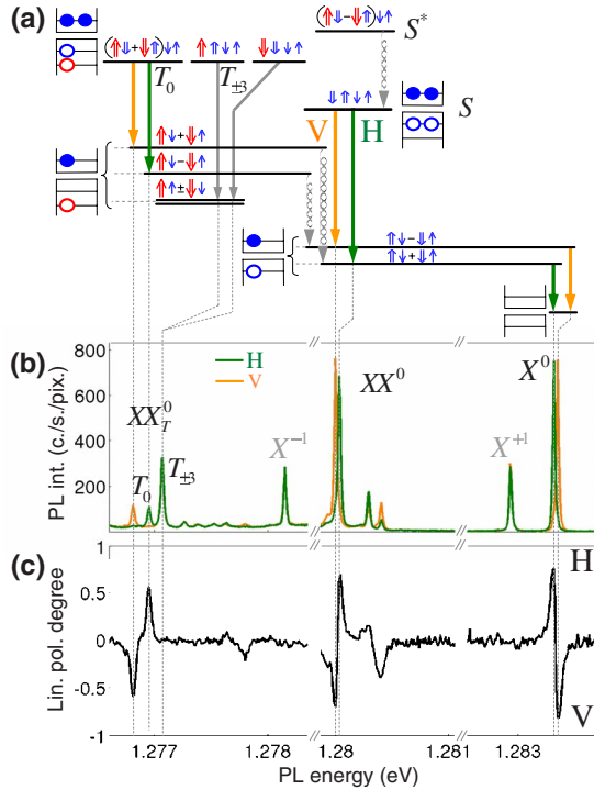
FIG. 1. (Color online) (a) Energy levels diagram for excitons and biexcitons in a neutral QD. Single-carrier level occupations are given along side each many-carrier level. The spin wave functions are depicted above each level. The symbol \uparrow ( \downarrow ) represents spin-up (spin-down) electron (hole). Short blue (long red) symbols represent charge carriers in the first (second) energy level. S ( S^* ) indicates ground (excited) biexciton hole-singlet state. T_0 ( T_{\pm 3} ) indicates the metastable spin-triplet-biexciton state with z -axis spin projection of 0 ( \pm 3 ). The solid (curly) vertical arrows indicate spin preserving (non)radiative transitions. Green (dark-gray) [orange (light-gray)] arrows represent photon emission in horizontal—H (vertical—V) polarization. (b) Polarized PL spectra. H (V) in green (orange). Spectral lines which are relevant to this work are marked and linked to the transitions in (a) by dashed lines. (c) Linear polarization spectrum. The value 1 (−1) means full H (V) polarization.
