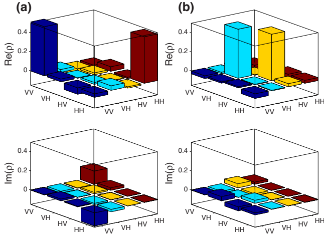
FIG. 3. (Color online) [(a) and (b)] Measured two-photon polarization density matrices for the ground-state (S) and spin-blockaded ( T_0 ) biexciton cascades, respectively, as obtained with spectral filtering. Real (imaginary) parts are shown in the top (bottom) panels. The Peres criterion (negativity of the partially transposed matrix) for the matrix in (a) [(b)] is 0.15 \pm 0.03 [ 0.05 \pm 0.1 ].
