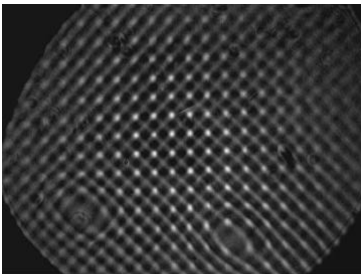
Crossed caustics from two acoustic waves. Notice two wave front errors below centre.
