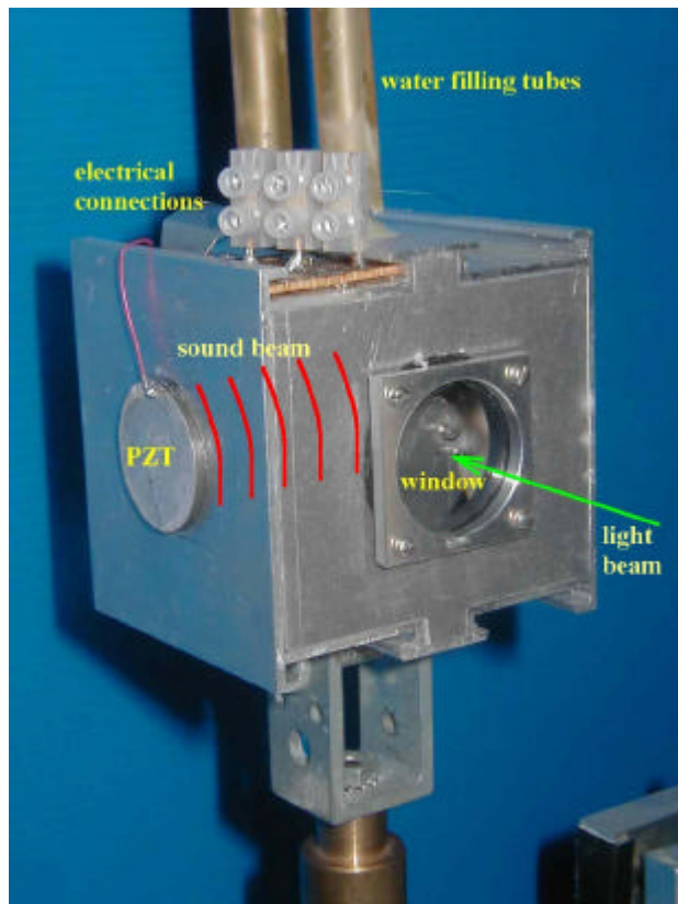
A standing sound wave modulates the light beam (horizontal beams)
